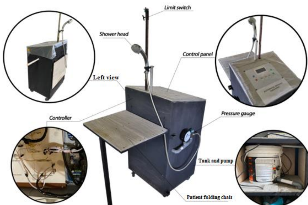
Figure 3. Automatic therapeutic shower prototype
