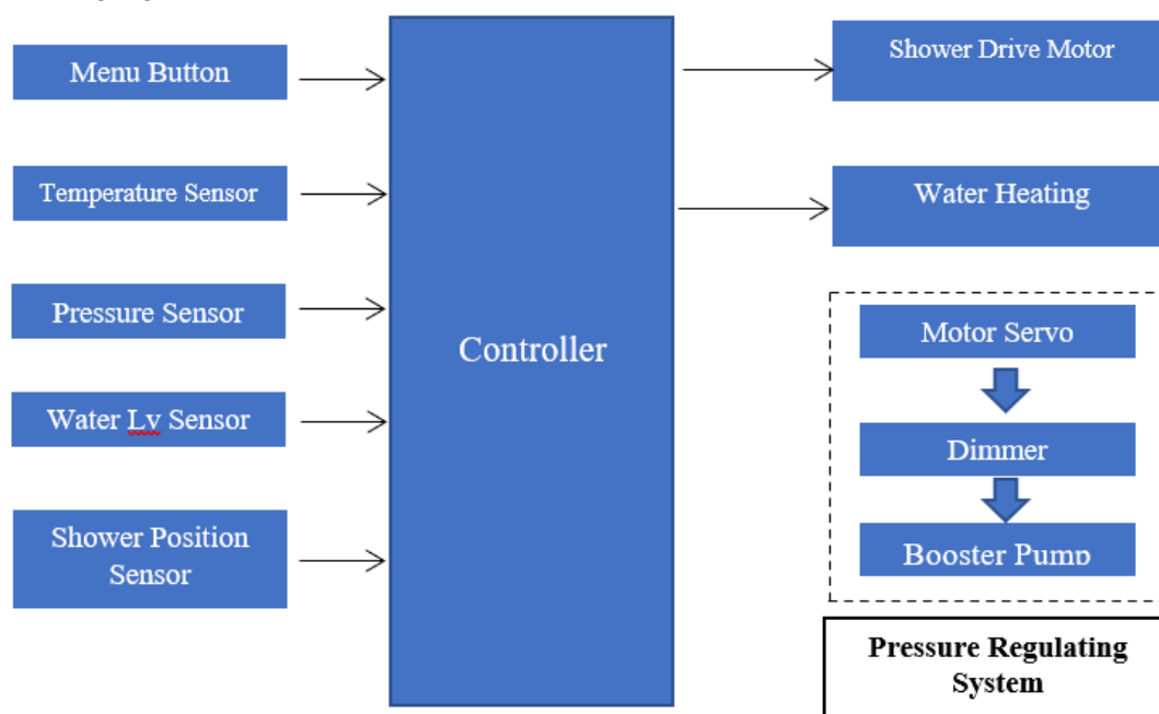
Figure 1. Work diagram of the shower therapy tool
